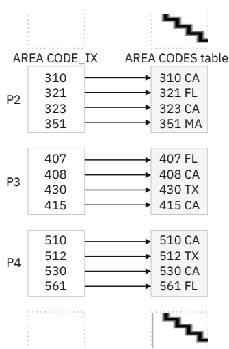
Figure 19. Partitioning index on the AREA_CODES table
