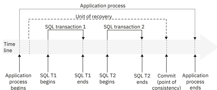
Figure 38. A unit of recovery within an application process
