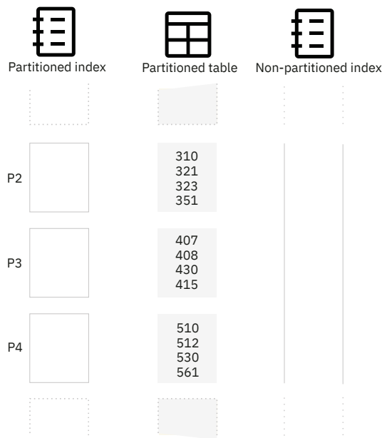
Figure 18. Comparison of partitioned and nonpartitioned index
